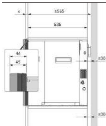
Fig. 9.5 Installation dimensions with 2 frame spacers
