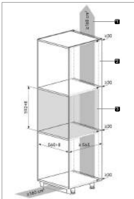
Fig. 9.1 Fitted unit
