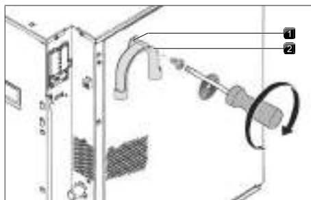
Fig. 9.10 How to fit the hook
