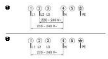
Fig. 9.15 Connection diagrams
