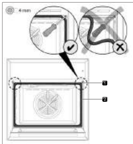
Fig. 9.17 Securing the appliance
