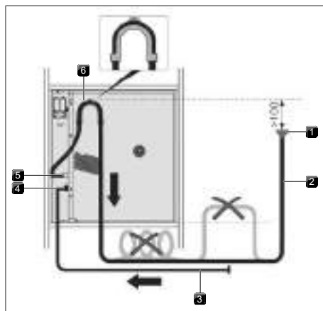
Fig. 9.13 Water drainage via hook
