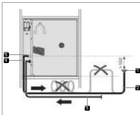
Fig. 9.12 Water drainage
