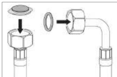
Fig. 9.14 Water inlet pipe with dirt filter and washer
