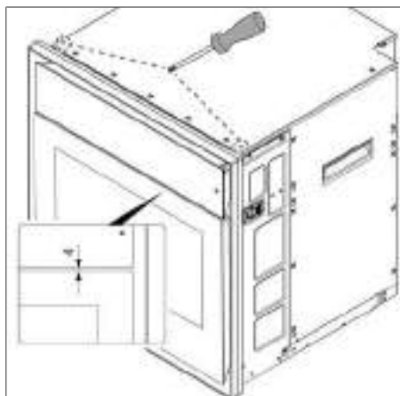
Fig. 9.16 Adjusting the distance between the operating unit and door
