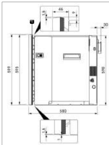
Fig. 9.2 Appliance dimensions
