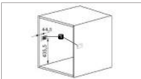
Fig. 9.9 Installation recess with unit mounting plates
