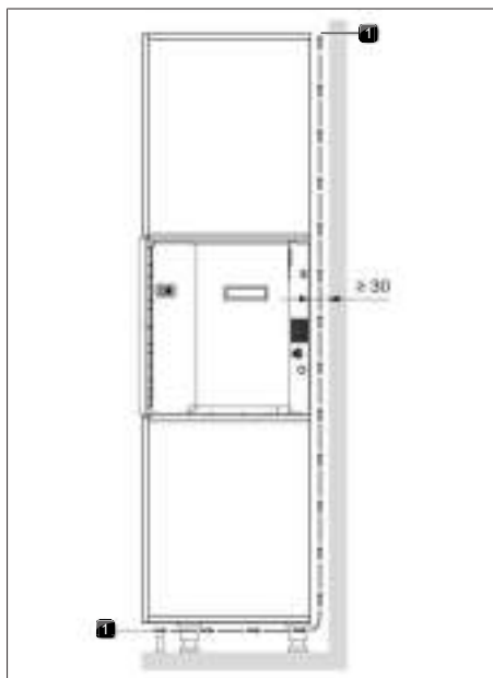
Fig. 9.18 Ventilation
