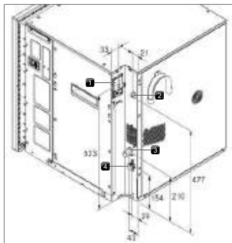
Fig. 9.11 Appliance connections
