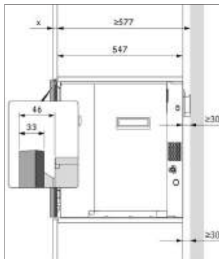
Fig. 9.4 Installation dimensions with 1 frame spacer
